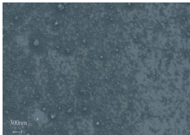
Q2 Fig. 1. SEM image of micelle-like structures in PS-P2VP/FeCl 3 hybrid film following chemical reduction. The average dimension of the nanoparticles is ~30 nm, (average value of distribution of diameters of 90% of nanoparticles).
