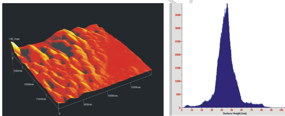
Fig. 2. AFM image of the PS-S2VP/FeCl 3 hybrid film. The typical surface roughness is ~45 nm for the scanned area of 1.7 \mu\text{m} \times 1.7 \mu\text{m} (average value of distribution of diameters of 90% of nanoparticles).
