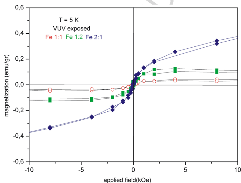
Fig. 10. Ferromagnetic responses at 5 K of the irradiated films with different iron concentrations for fields up to 10 kOe. The coercivities up to 1.2 kOe are 99, 74 and 60 Oe for iron ratios of 2:1, 1:1 and 1:2 respectively.
